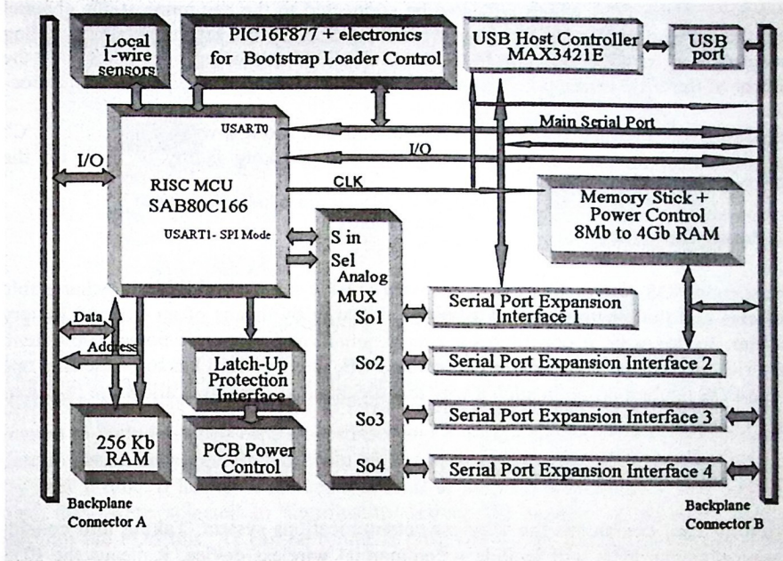
Figure 3. Preliminary block diagram for the PDS computer.
