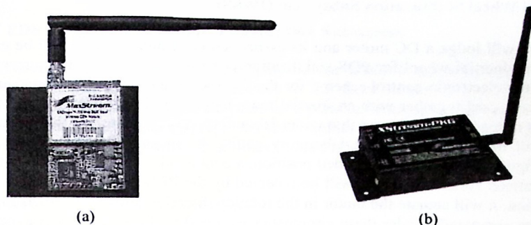
Figure 4. RF radio modem being considered for the project, a) For a PDS PCB and, b) For ground station.
